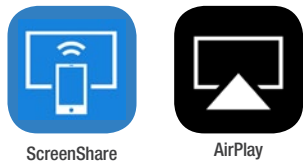
ScreenShare
